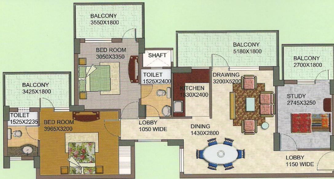
3 BEDROOM UNIT PLAN - AREA - 1460 SQ.FT.
